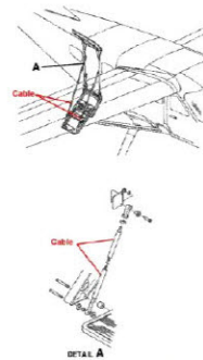
Cable Assembly Installation S2837-1EH or S2837-2EH
