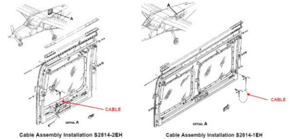
Cable Assembly Installation S2814-2EH
